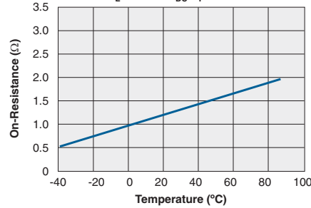
Typical On-Resistance vs. Temperature ( I_L=100mA_{DC}, I_F=10mA )
